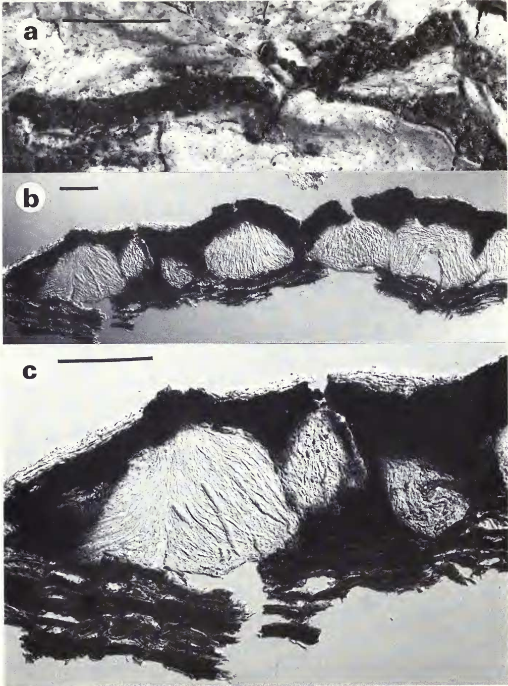
Fig. 33 Celothelium cinchonarum (Müll. Arg.) Vainio (G-holotype) (a) Surface view of ascomata; scale = 500 µm; (b), (c) Vertical section of ascomata showing pseudostroma; scale = 100 µm.
